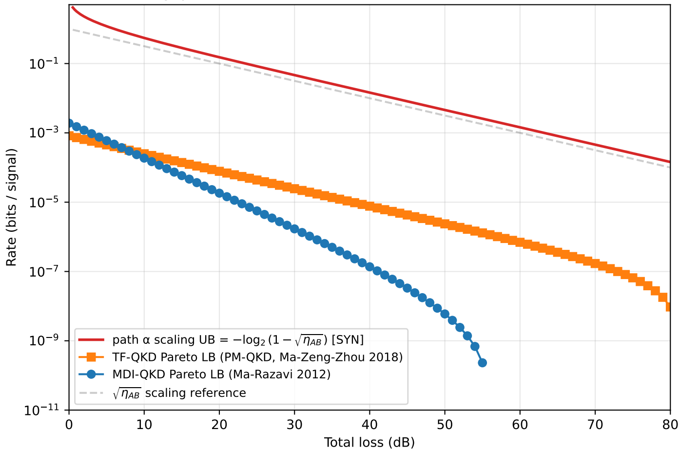
Path \alpha v0.2 §3.1 — scaling UB vs Pareto LB (numerical reframing only) [SYN] sub-gaps \propto G1/G2/G2.E/G3 OPEN; no Lemma A/B/C closure asserted
