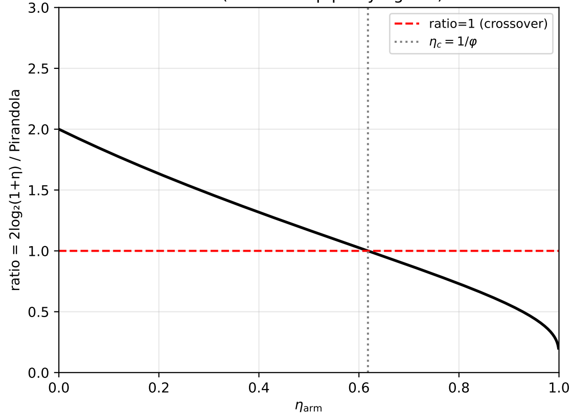
Ratio (below 1 = \beta proxy tighter)
