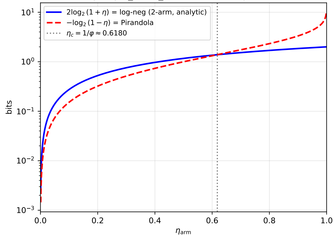
log-neg( E_1 \otimes E_2 ) vs Pirandola (qubit AD)
