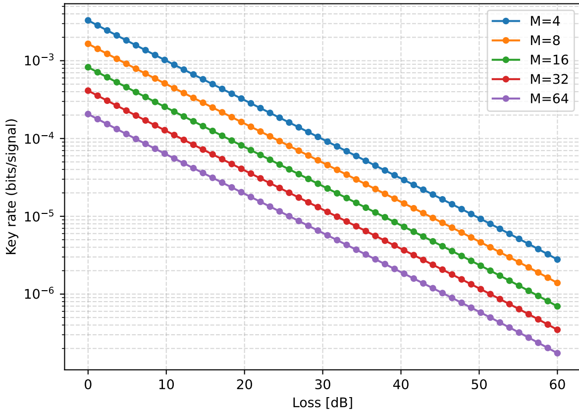
PM-QKD: effect of phase-slice count M on rate
