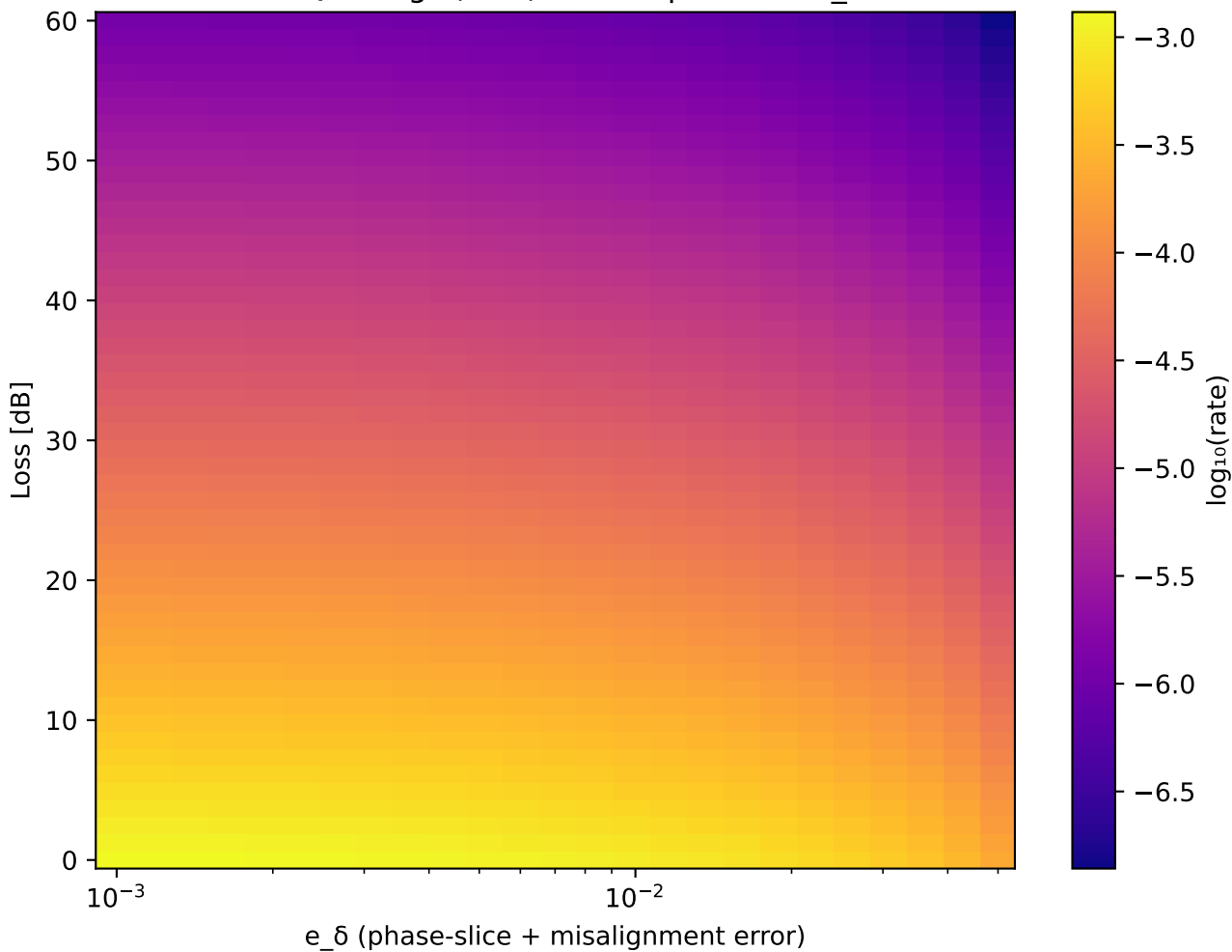
PM-QKD \log_{10}(\text{rate}) heatmap: \text{loss} \times e_{\delta}
