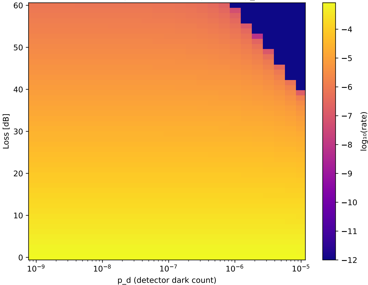
PM-QKD \log_{10}(\text{rate}) heatmap: \text{loss} \times p_d
