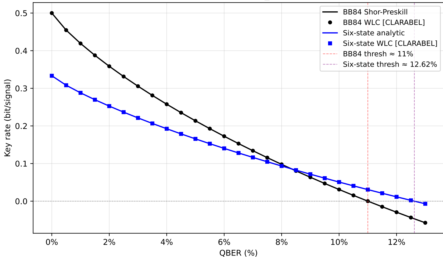
BB84 vs Six-State ( f_{ec}=1.0 )
