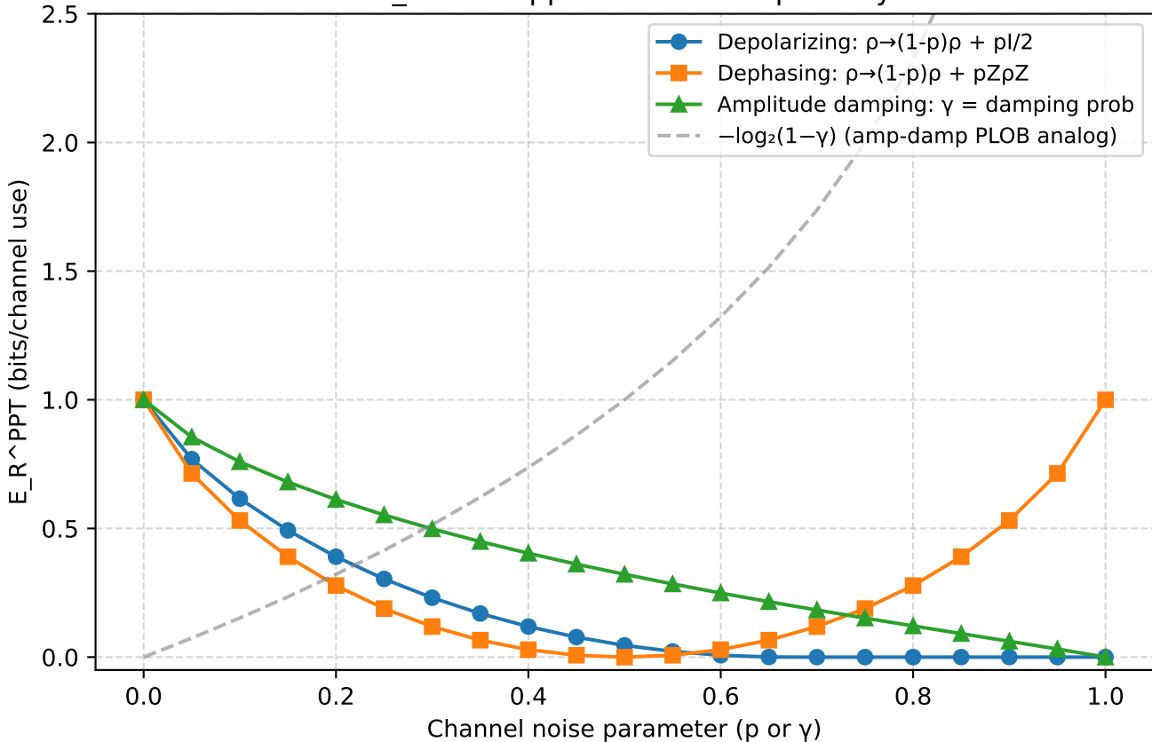
Numerical E_R^{\text{PPT}} upper bounds for qubit toy channels
