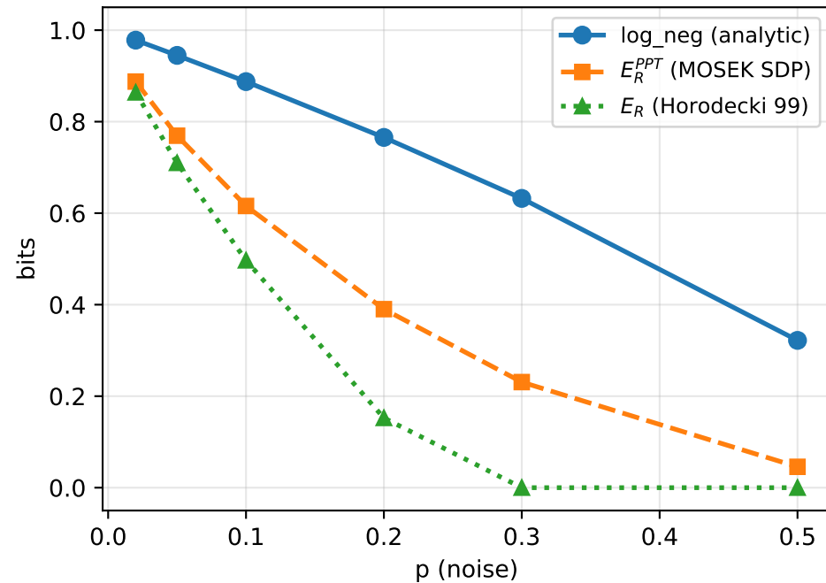
Depolarizing
