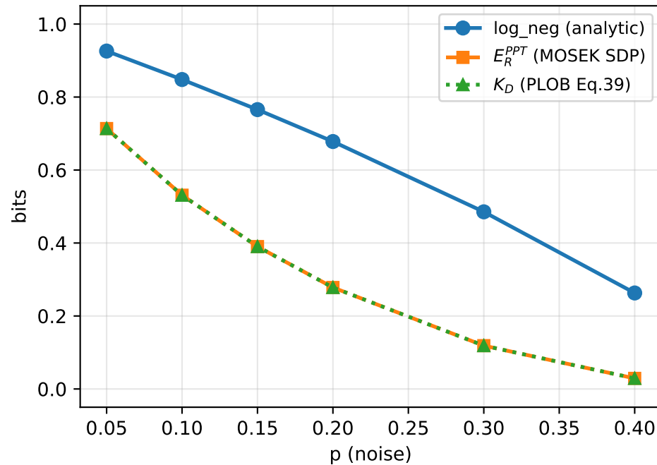
Dephasing
