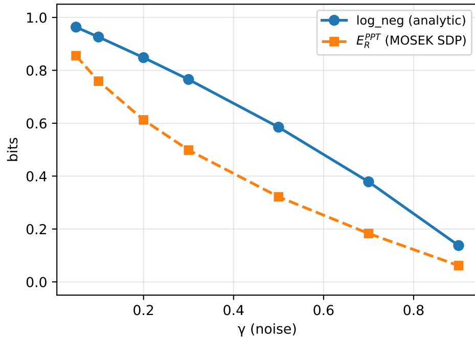
Amplitude Damping
