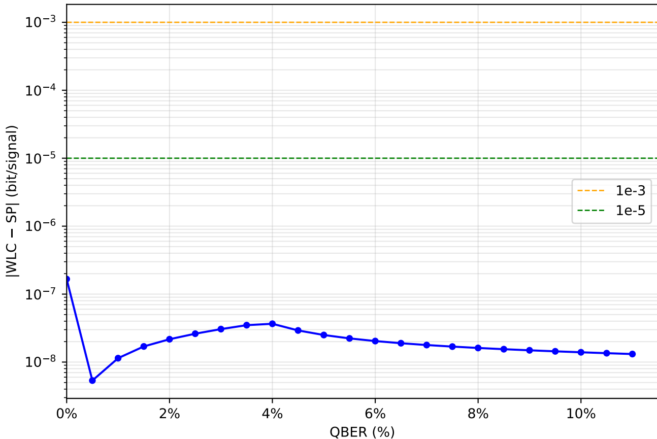
WLC vs Shor-Preskill — absolute deviation
