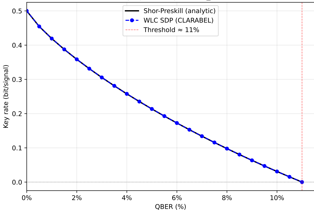
BB84 Asymptotic Key Rate ( f_{ec} = 1.0 )
