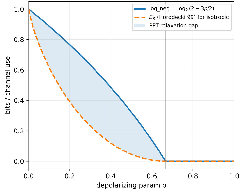
Qubit Depolarizing: log_neg vs E_R (analytic)
