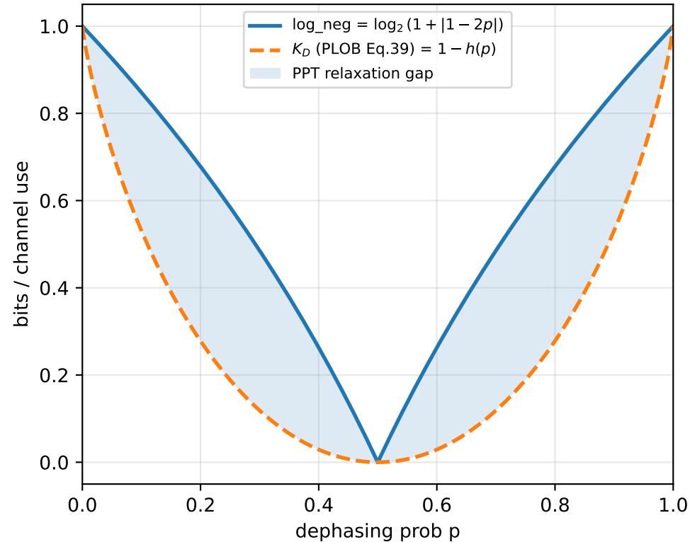
Qubit Dephasing: log_neg vs K_D (PLOB exact)
