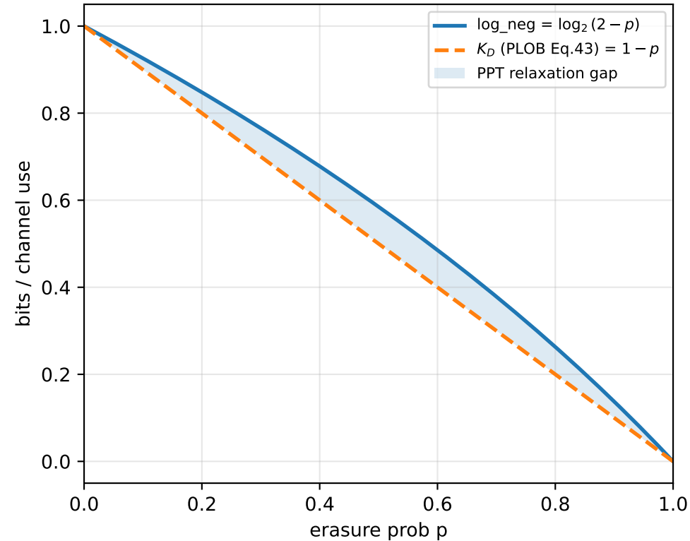
Qubit Erasure: log_neg vs K_D (PLOB exact)
