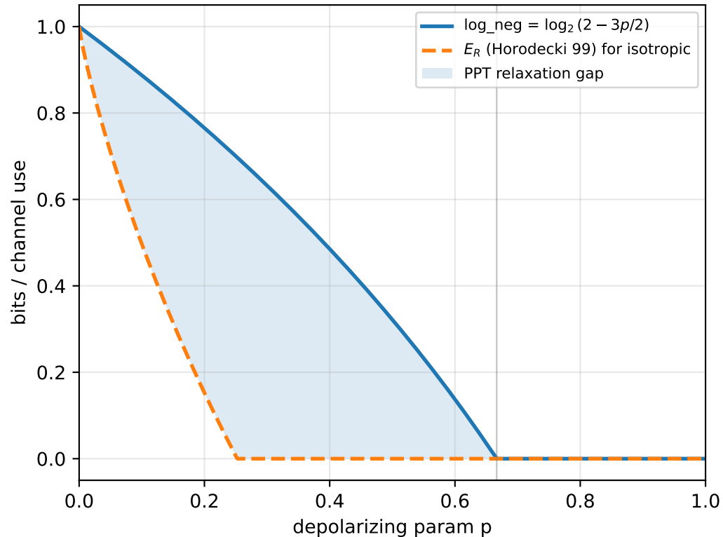
Qubit Depolarizing: log_neg vs E_R (analytic)
