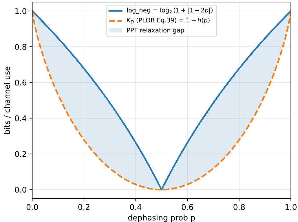
Qubit Dephasing: log_neg vs K_D (PLOB exact)
