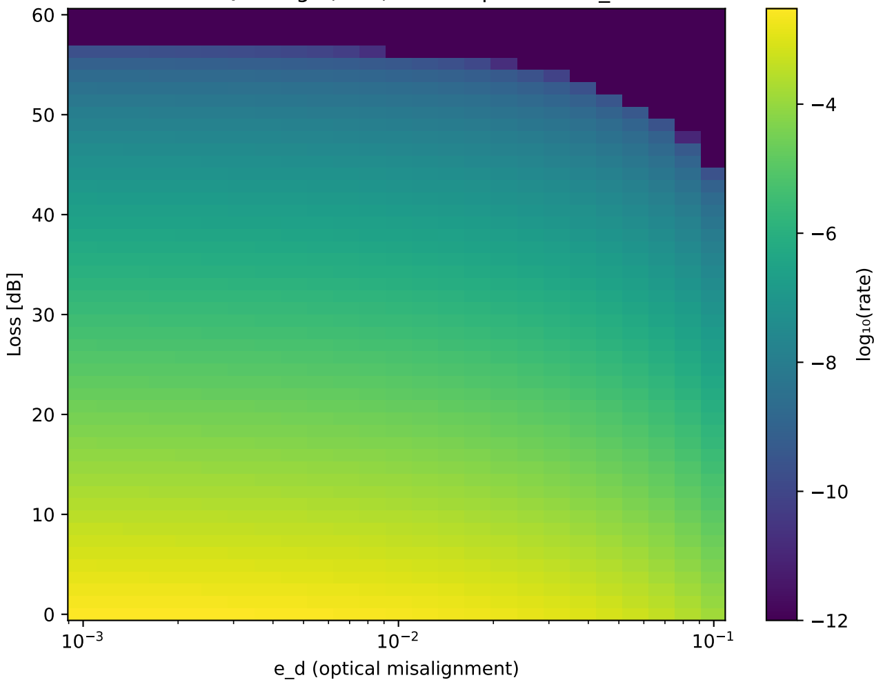
MDI-QKD \log_{10}(\text{rate}) heatmap: \text{loss} \times e_d
