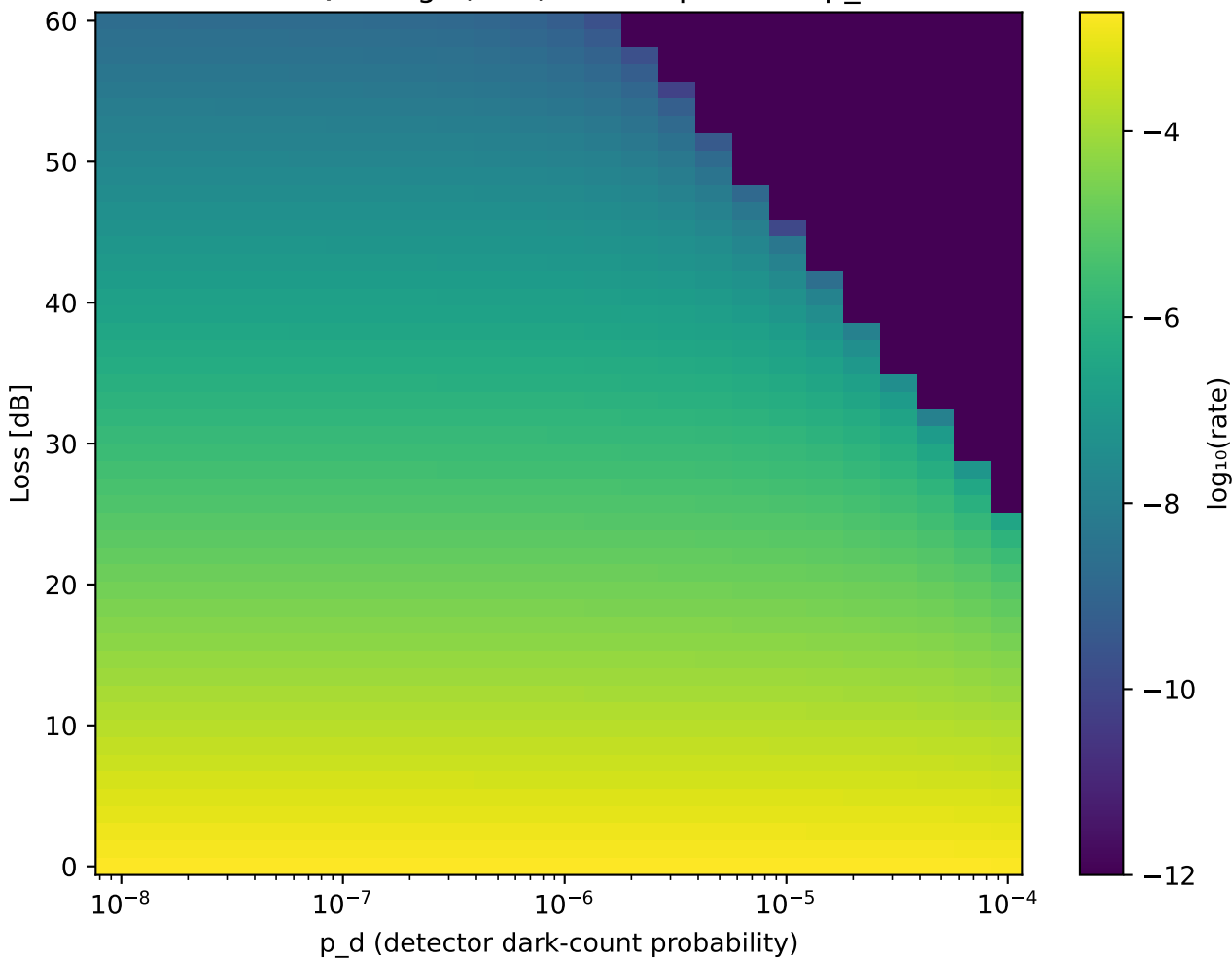
MDI-QKD \log_{10}(\text{rate}) heatmap: \text{loss} \times p_d
