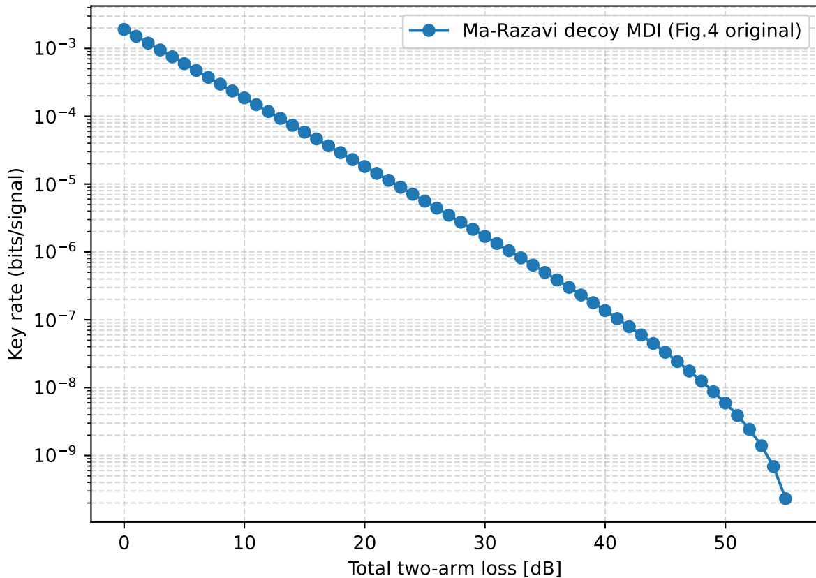
MDI-QKD: rate vs loss (Ma-Razavi 2012 Table I defaults)
