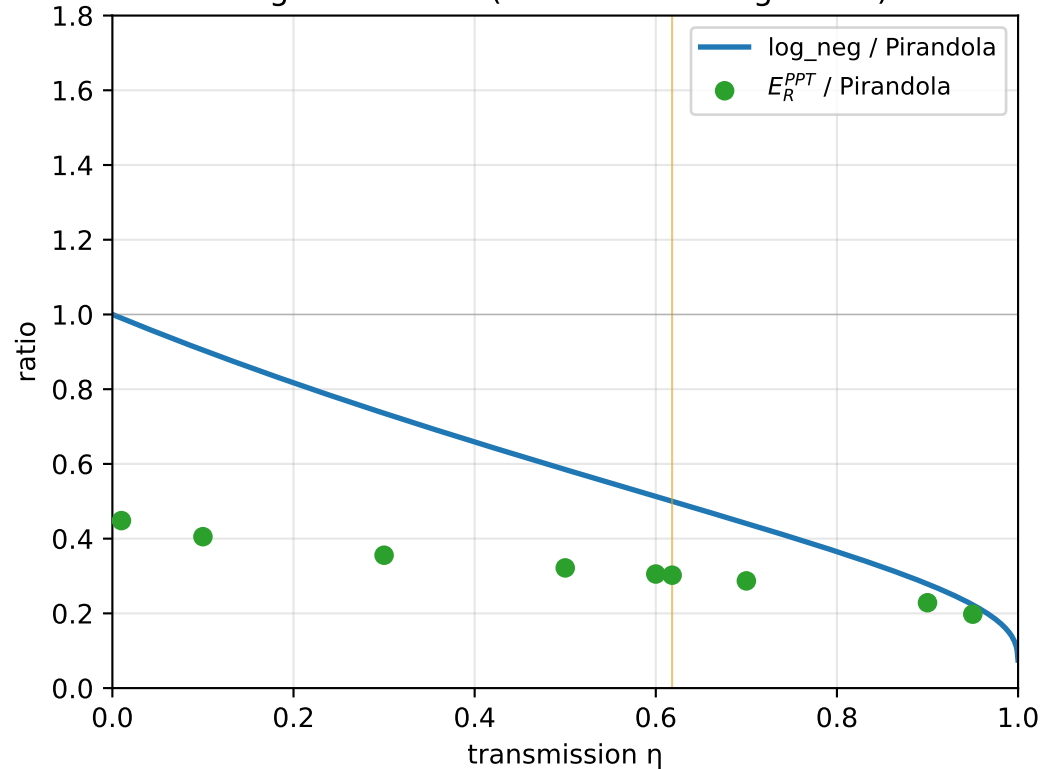
Tightness ratio (vs Pirandola single-arm)
