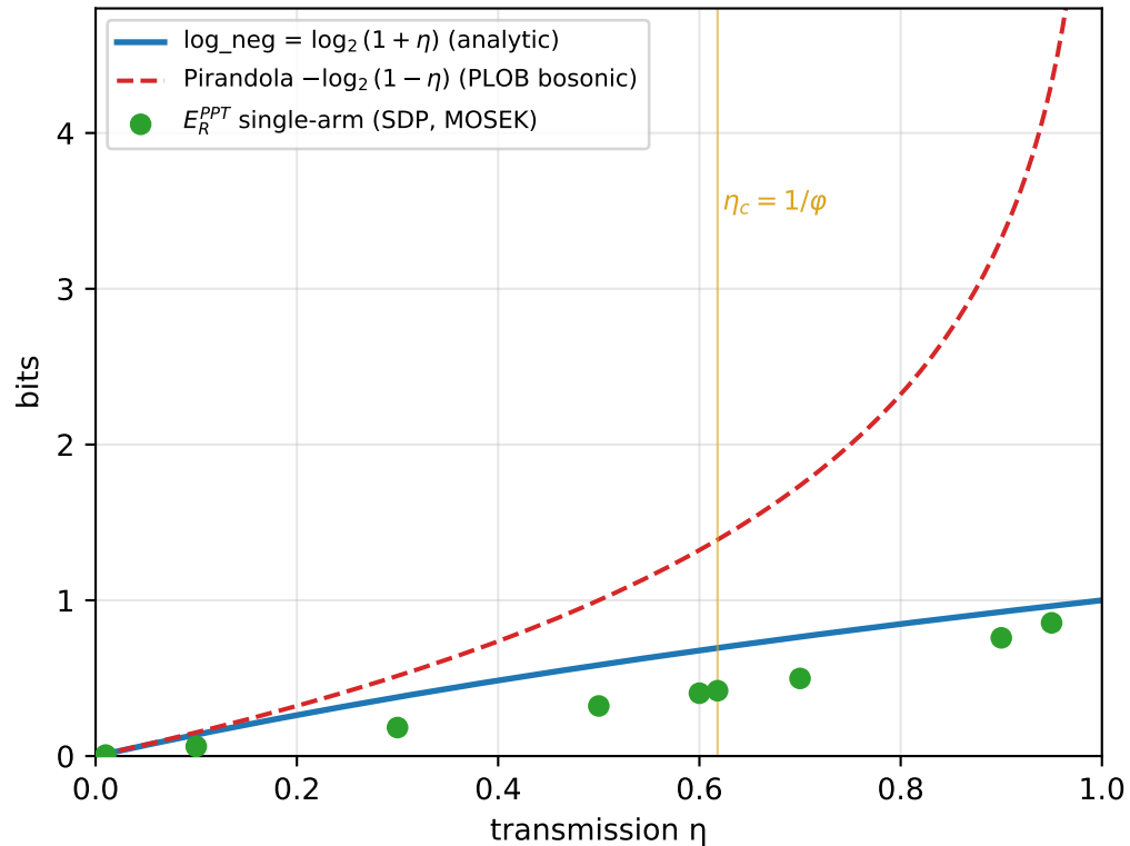
AD channel: \log\_neg vs E_R^{PPT} vs Pirandola (single arm)
