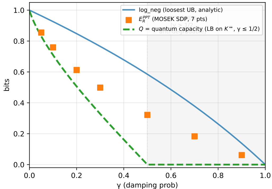
AD: channel Q (LB on K^\leftrightarrow ) + Choi-state E_R^{PPT} / \log\_neg (AD not tele-covariant; Choi-state values NOT automatic channel UB)
