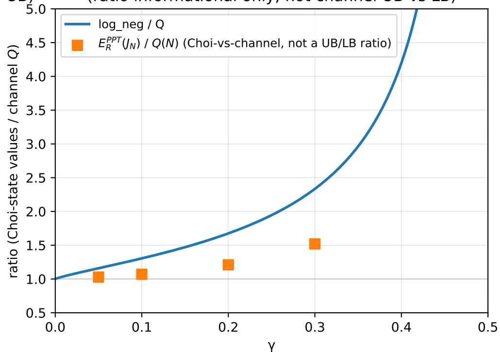
AD: Choi-state \log\_neg and E_R^{PPT} compared to channel Q (ratio informational only; not channel UB vs LB)
