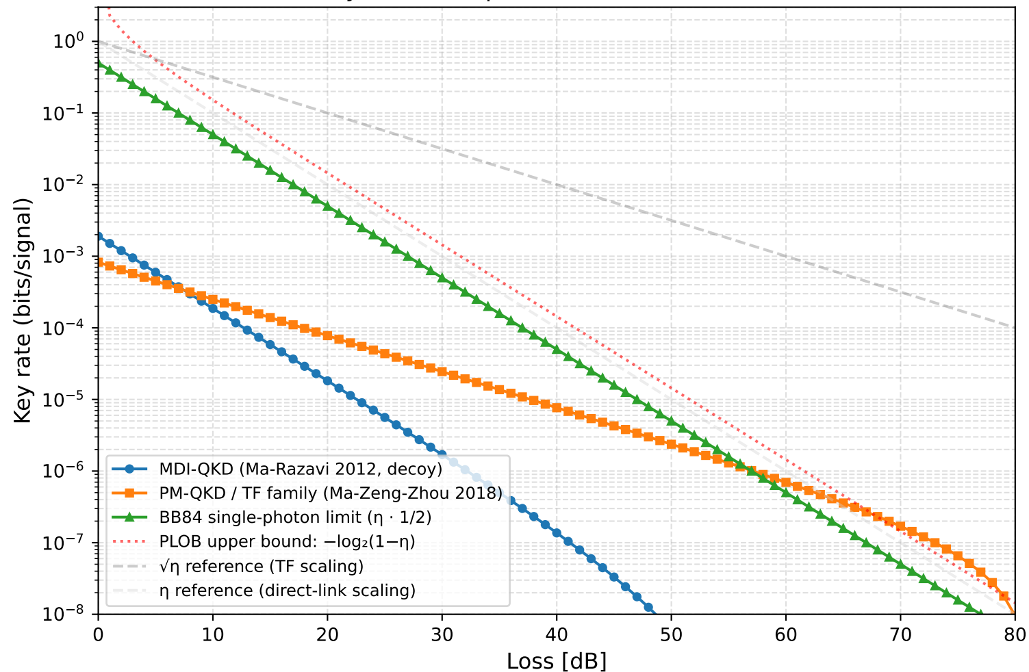
DV-QKD Family Pareto Map: BB84 / MDI-QKD / PM-QKD vs PLOB
