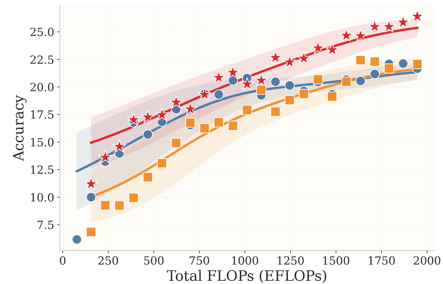
Tasks Average
