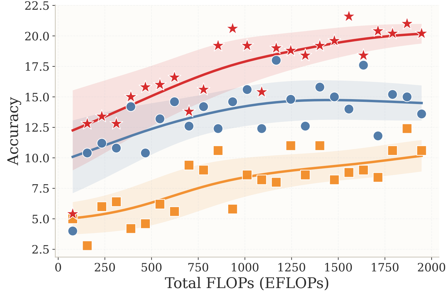
SQuAD
