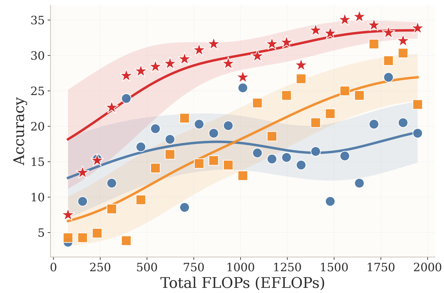
HellaSwag
