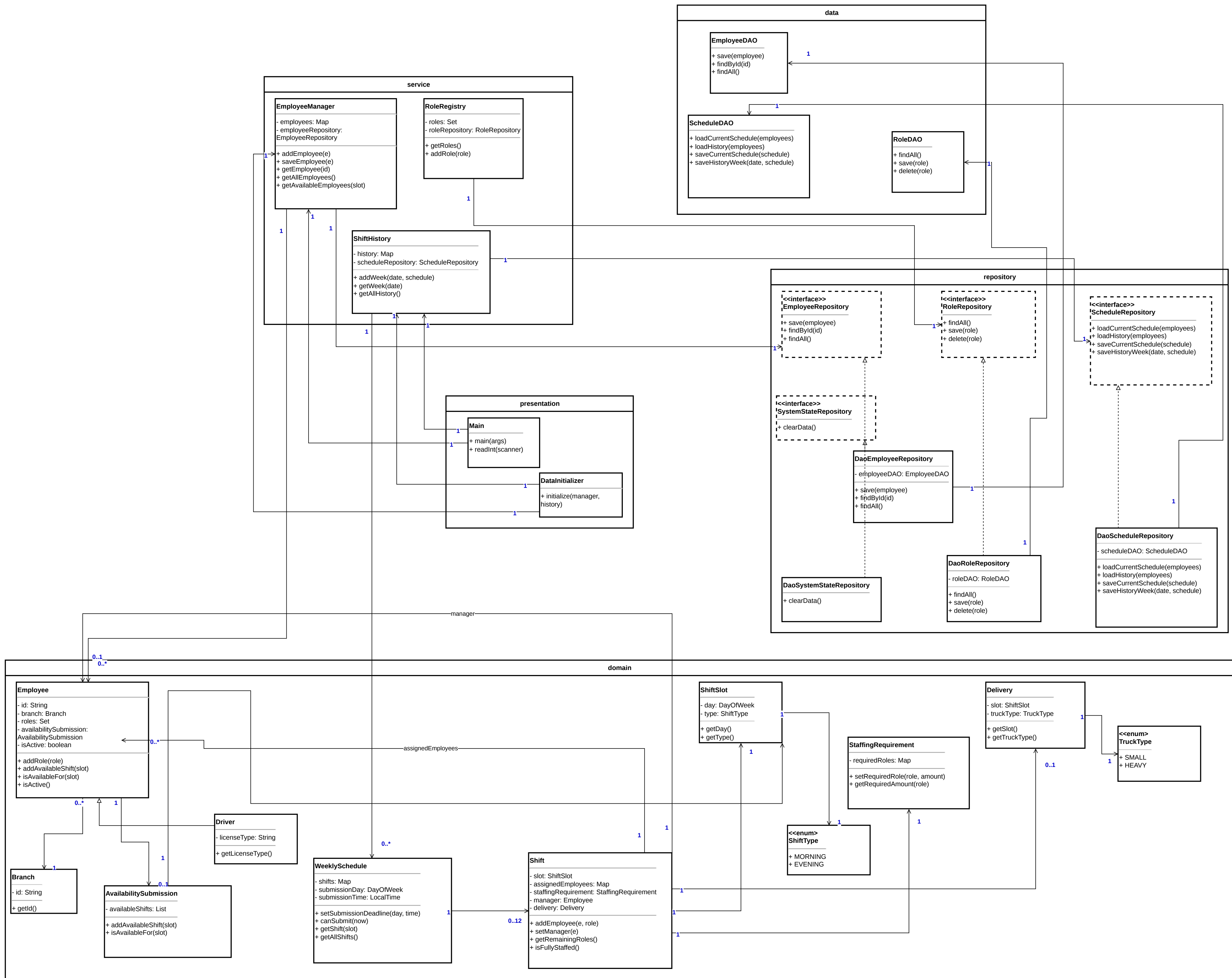
SuperLi System - UML Class Diagram
