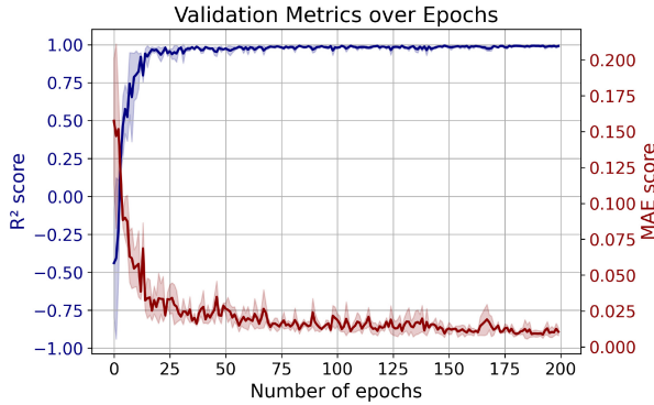
Fig. 10. Learning curve for fault probability prediction on tree-shaped service meshes: validation R^2 score (left axis) and validation MAE score (right axis) over epochs (mean \pm standard deviation across 3 runs).
