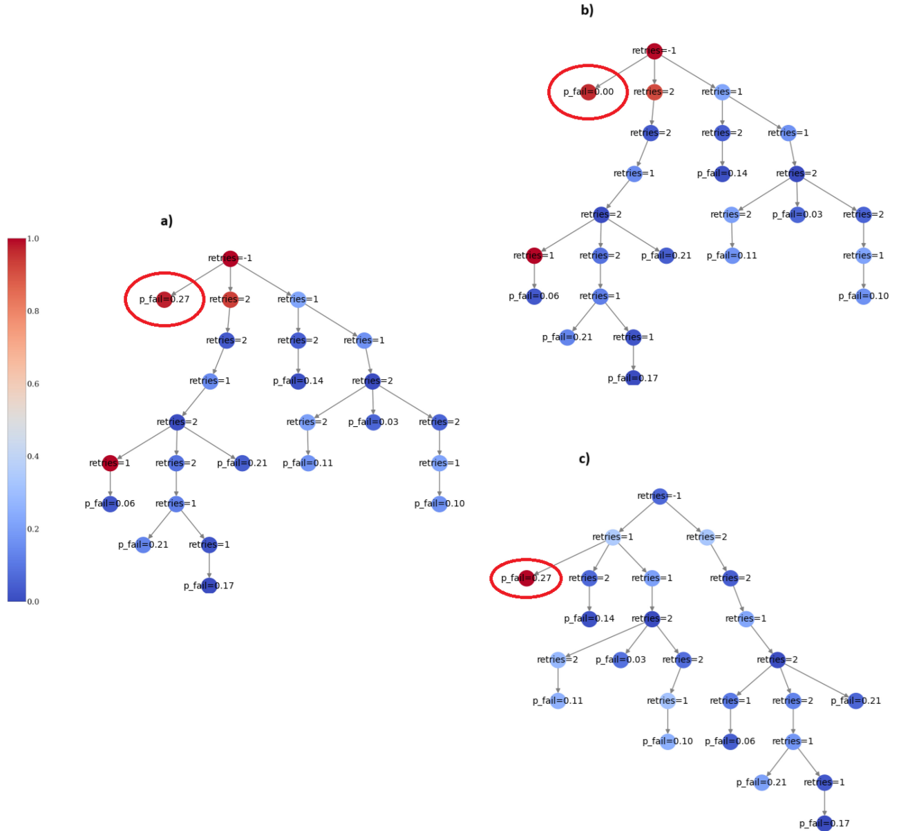
Fig. 14. Demonstration of explainer network on a service mesh. (a) A critical leaf node with high 0.27 failure probability near the root leads to a predicted system fault probability of 0.94, closely matching the ground truth of 0.93. (b) Setting the failure probability of the critical node to 0.00 reduces the predicted system fault probability to 0.00. (c) Moving the critical node lower in the tree, the predicted system fault probability drops to 0.01 due to the intermediary node's recovery ability.
