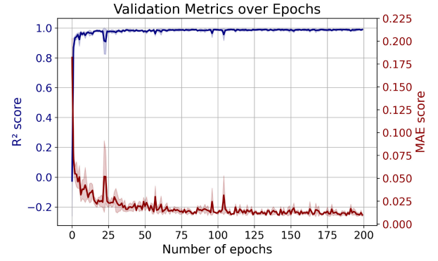
Fig. 8. Learning curve for fault probability prediction on tree-shaped service meshes: validation R^2 score (left axis) and validation MAE score (right axis) over epochs (mean \pm standard deviation across 3 runs).
