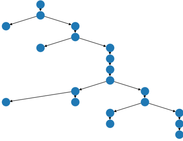
Fig. 3. Simple service mesh application topology.
