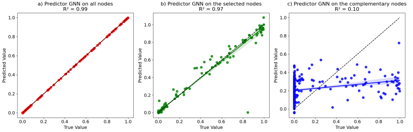
Fig. 12. Regression plots for fault probability prediction on tree-shaped service meshes using the predictor GNN: a) Predictions on 100% of the nodes, closely aligned with the ground truth values, achieving an R^2 score of 0.992, indicating excellent predictive performance; b) Predictions using the selected 30% of nodes (chosen by the explainer network), maintaining strong performance with an R^2 score of 0.974, confirming that these nodes are critical for predicting system-level fault probabilities and capturing most of the variance in the system; c) Predictions using the complementary 70% of unselected nodes, with an R^2 score of 0.104, demonstrating that these nodes provide little information about the system-level fault probabilities, essentially resulting in a baseline mean prediction. This clearly demonstrates the algorithm’s success in identifying critical components, as the selected nodes retain most of the variance while the unselected ones provide minimal predictive value.
