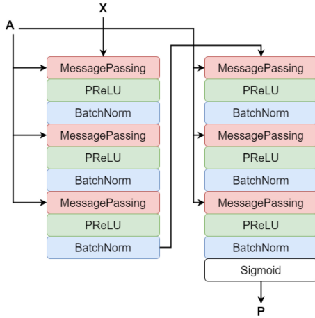
Fig. 7. The explainer network consists of six message-passing blocks, followed by a sigmoid layer that generates a probability distribution over the nodes, reflecting their importance for fault probability prediction.
