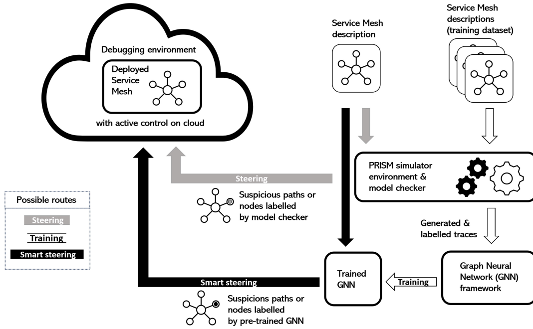
Fig. 2. Proposed framework for debugging cycle with tools and dataflow.
