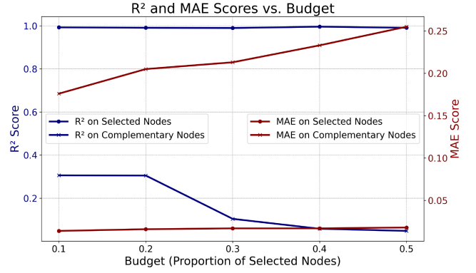
Fig. 13. R^2 and MAE Scores vs. Budget (Proportion of Selected Nodes): As the selection budget increases from 10% to 50%, the R^2 score for selected nodes remains consistently high (between 0.991 and 0.996), demonstrating that even small subsets capture most of the predictive information. In contrast, the R^2 score for complementary nodes steadily decreases from 0.306 to 0.048 as more informative nodes are moved to the selected set. Similarly, the MAE score for selected nodes remains low, while the MAE score for complementary nodes increases, reinforcing the importance of the selected nodes in system fault probability prediction.
