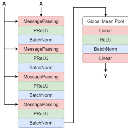
Fig. 5. The proposed GNN architecture for fault probability prediction.
