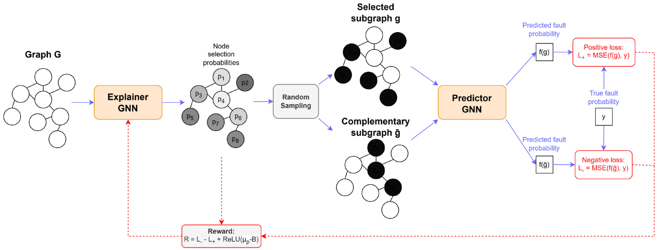
Fig. 6. Illustration of training the explainer GNN for identifying critical components in the service mesh. The explainer GNN generates probabilities for node masking, producing a mask that selects the most important nodes for fault probability prediction. The predictor GNN then evaluates the selected subgraph g and its complementary \bar{g} . If the mask captures the most relevant nodes, the predictor's performance on the subgraph g should closely match its performance on the original graph, while its performance on the complementary subgraph \bar{g} should drop significantly, confirming that the selected nodes are necessary and sufficient for the prediction. The mean of the probabilities, \mu_p , and the budget B (e.g., B = 33\% means one-third of the nodes are retained) control the number of nodes selected.
