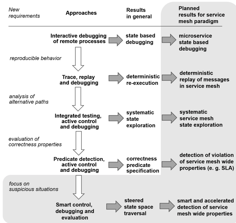
Fig. 1. Classification of general distributed debugging methodologies [8] extended with our planned results in service mesh environment (grey background).
