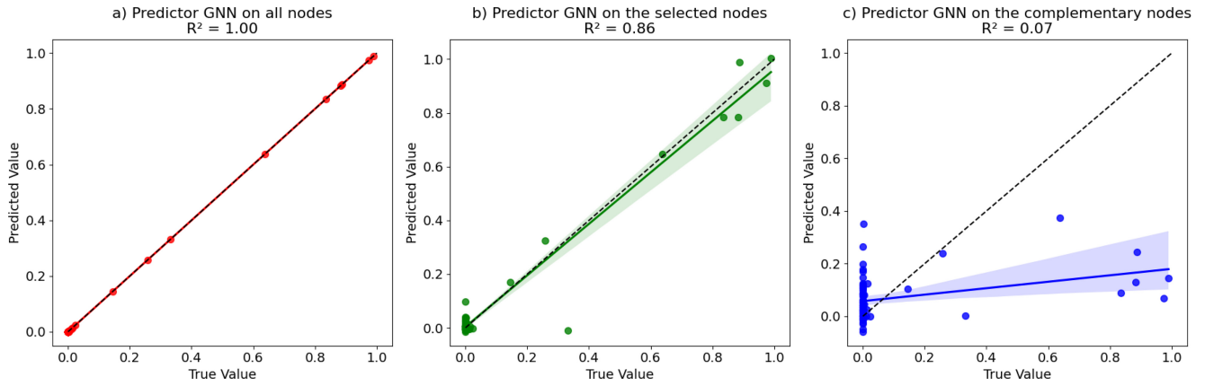
Fig. 15. Regression plots for fault probability prediction on DAG-shaped service meshes using the predictor GNN: (a) Predictions on 100% of the nodes, achieving an R^2 score of 0.996, indicating excellent predictive performance; (b) Predictions using the selected 30% of nodes (chosen by the explainer network), achieving an R^2 score of 0.861, showing that these nodes capture most of the critical information for fault probability prediction; (c) Predictions using the complementary 70% of nodes, achieving an R^2 score of 0.072, demonstrating that these nodes provide little to no value for predicting fault probabilities.
