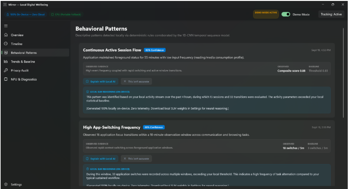
Figure 2: Behavioral Patterns View featuring on-device SLM RAG explanation over 4-hour SQLite history and active threshold recalibration.
