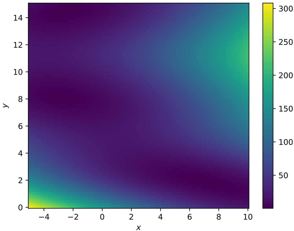
2D Branin Function
