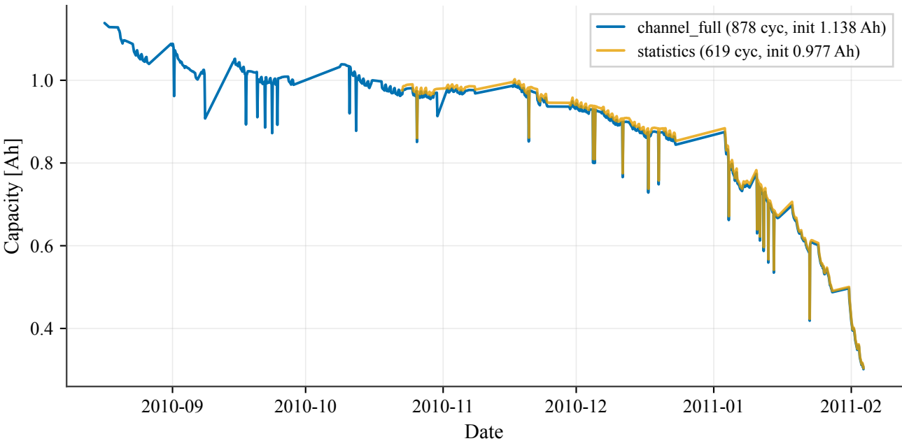
CALCE CS2_35 candidate timelines
