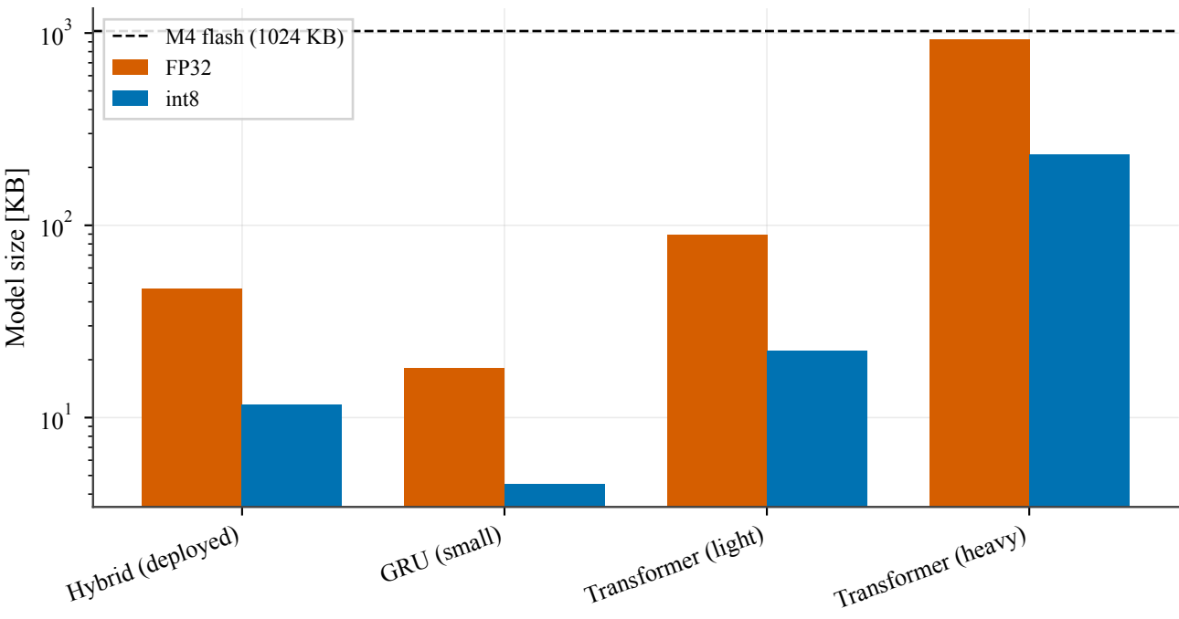
Footprint vs. Cortex-M4 flash budget
