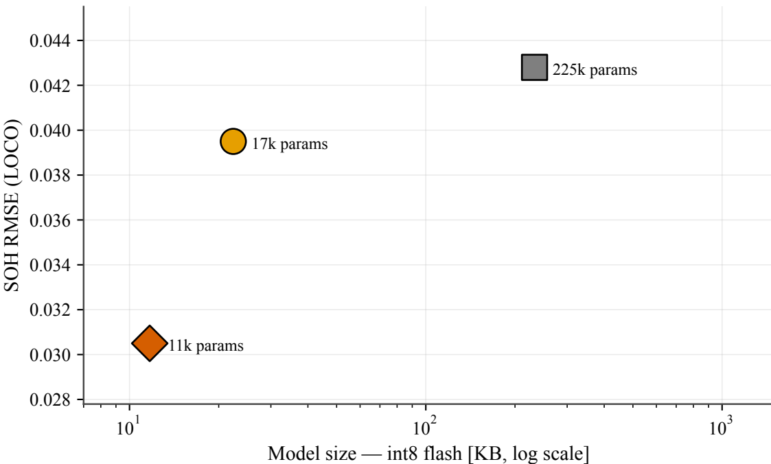
Accuracy vs. memory (lower-left is better)
