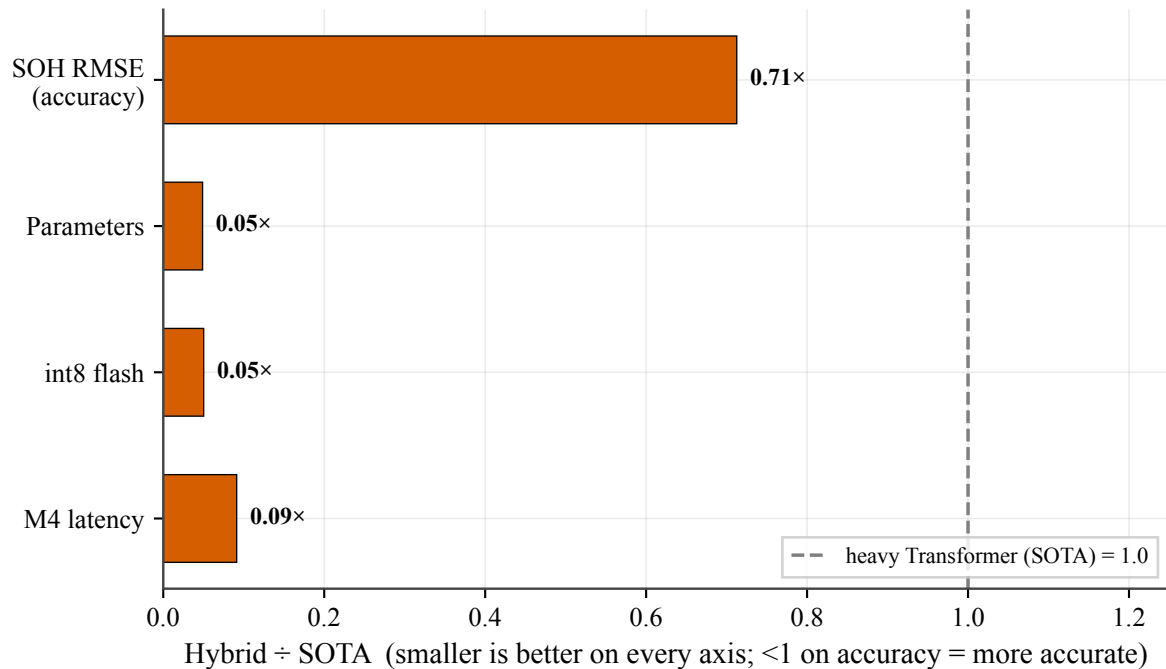
Deployed Hybrid relative to SOTA
