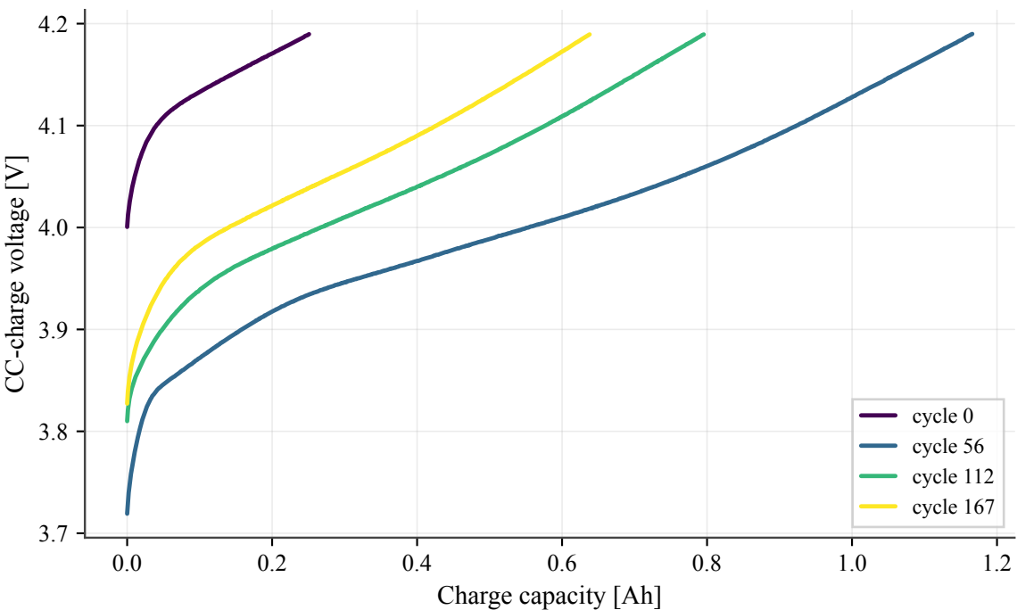
NASA B0005 CC-charge V-Q curves vs. aging
