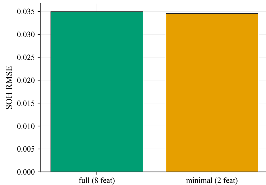
Feature-set ablation
