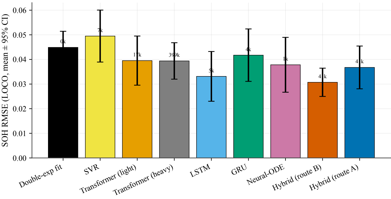
SOH accuracy benchmark (NASA LOCO)
