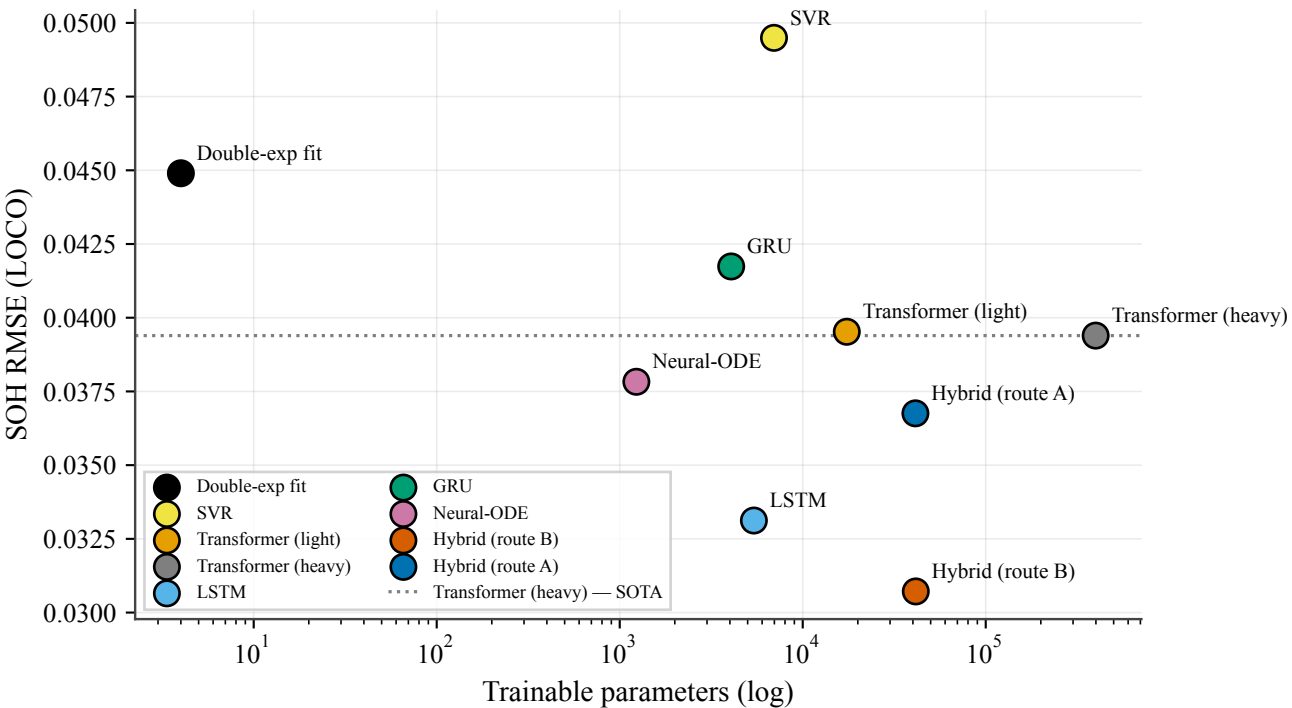
Accuracy vs. model size (LOCO)
