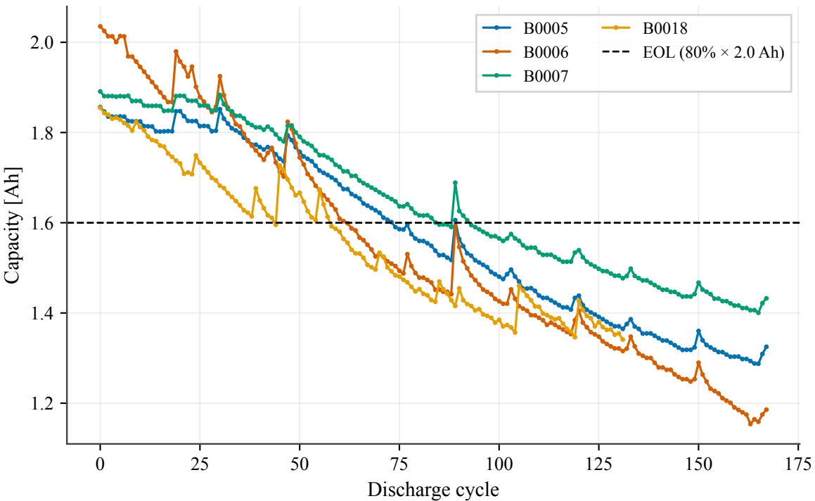
NASA capacity fade (four LCO 18650 cells)
