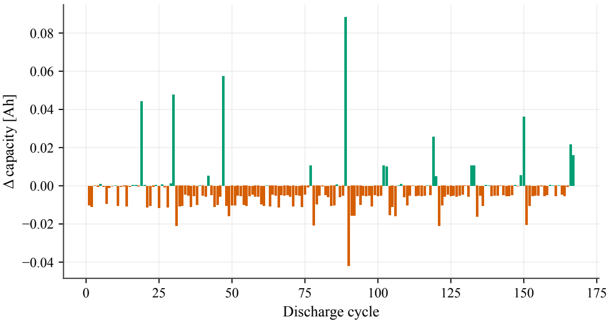
B0005 cycle-to-cycle capacity change
