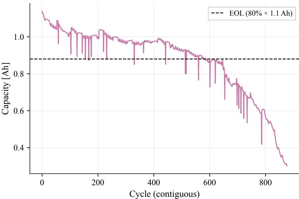
CALCE CS2_35 capacity fade
