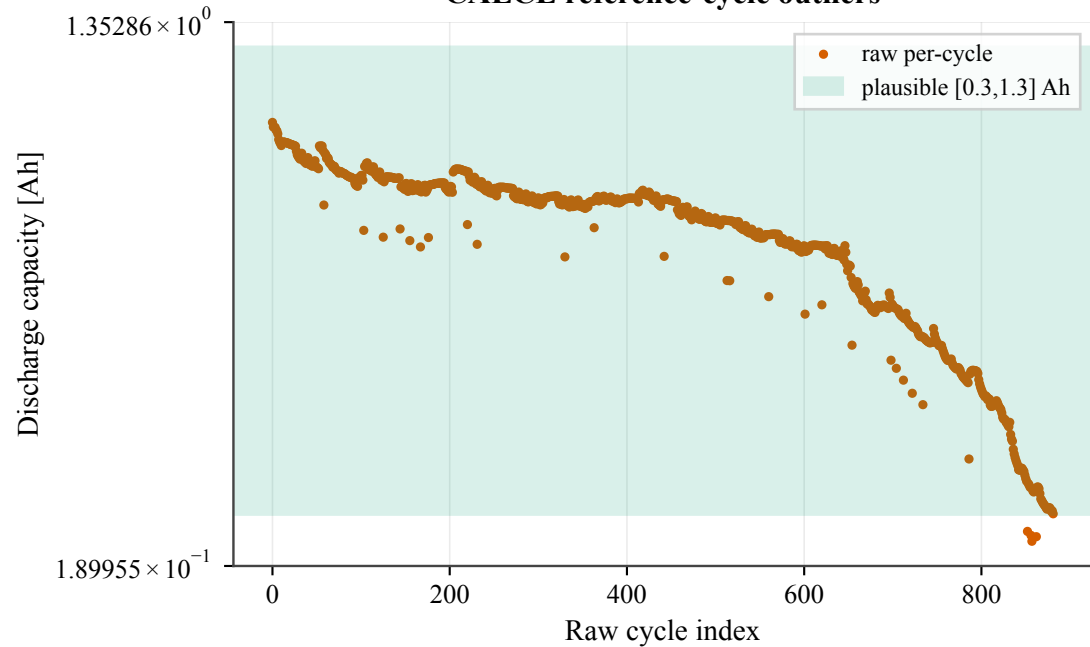
CALCE reference-cycle outliers
