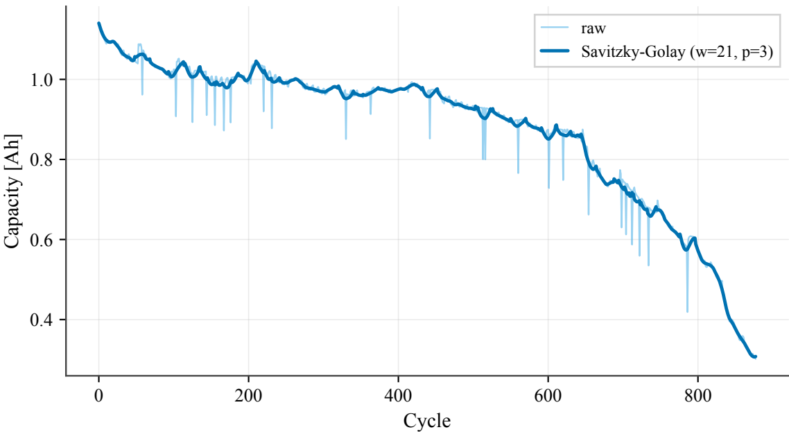
CALCE capacity: raw vs. Savitzky-Golay
