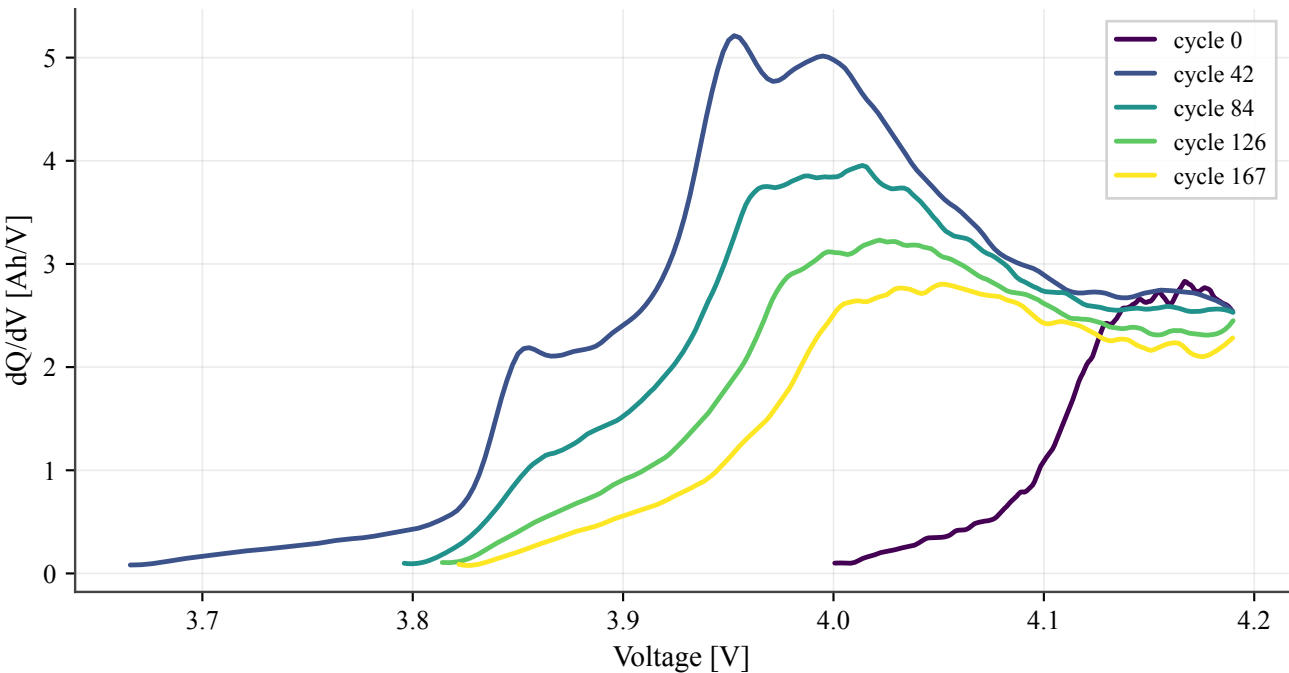
NASA B0005 ICA (dQ/dV) evolution with aging
