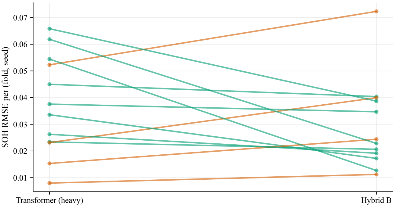
Paired comparison: Hybrid B vs. Transformer (heavy)
