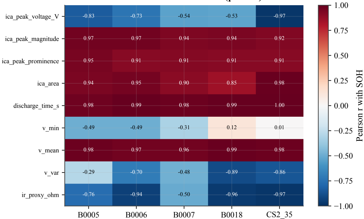
Feature → SOH correlation (per cell)
