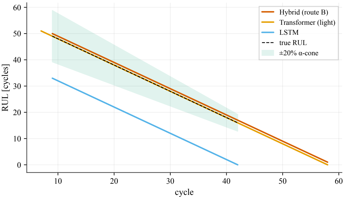
\alpha - \lambda prognostic accuracy (B0018)
