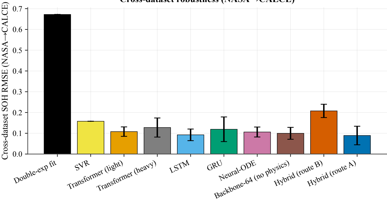
Cross-dataset robustness (NASA→CALCE)
