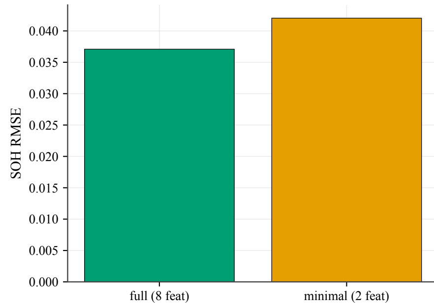
Feature-set ablation
