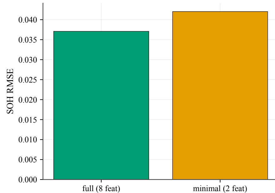
Feature-set ablation
