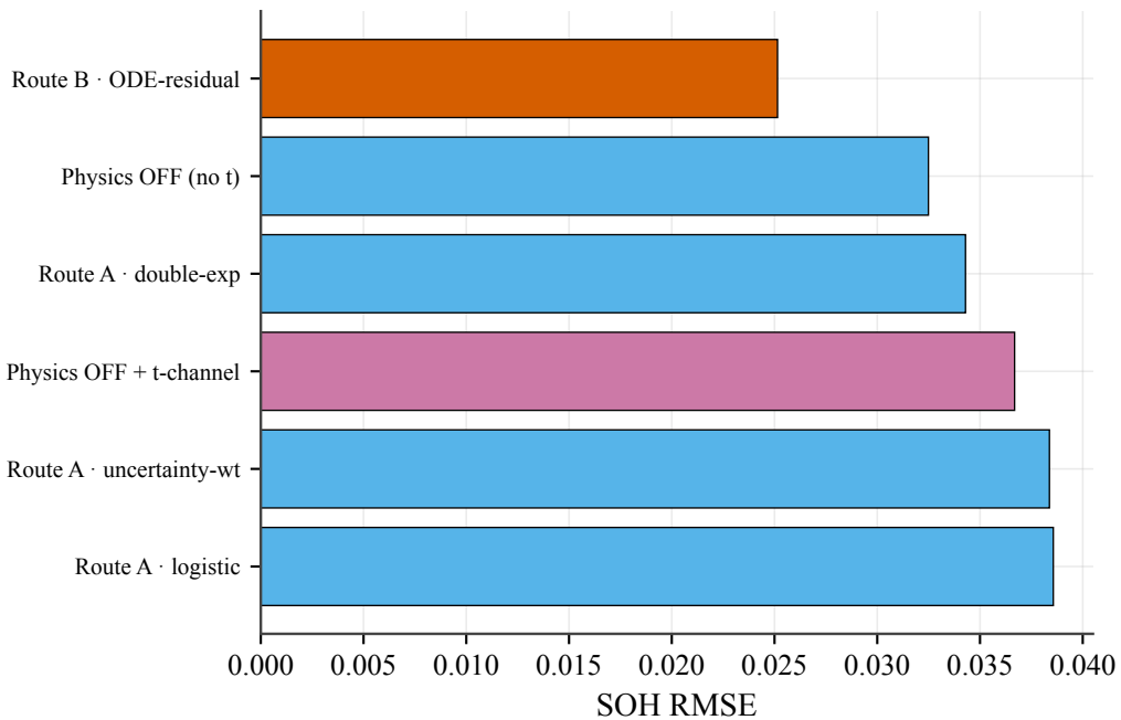
Design ablation
