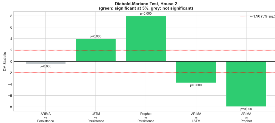
Figure 11. Diebold-Mariano statistics for House 2. Green bars are significant at the 5 percent level ( |DM| > 1.96 ); grey bars are not. The ARIMA versus Persistence comparison is the only non-significant pair.
