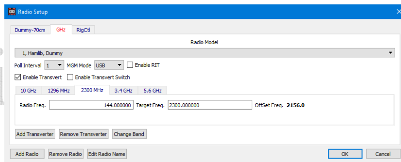
Figure 78 – Transverter definition
