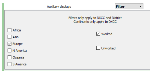
Figure 28 – Statistics Filter
