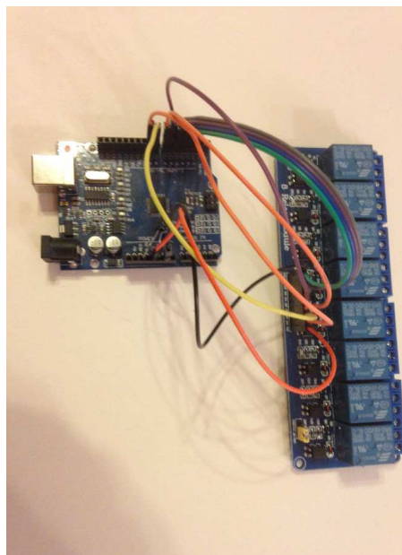
Figure 131 – Arduino and Relay Board
