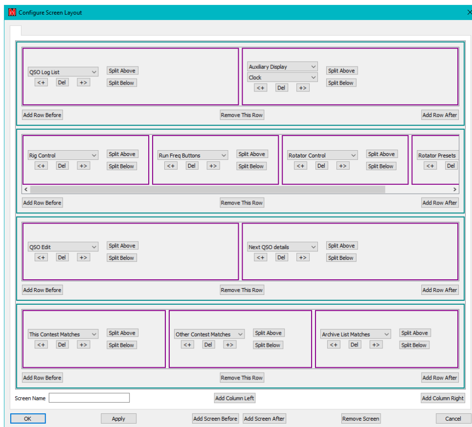
Figure 52 – Default screen layout configuration
