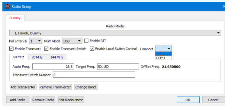
Figure 101 – Defining Local Switch Control port
