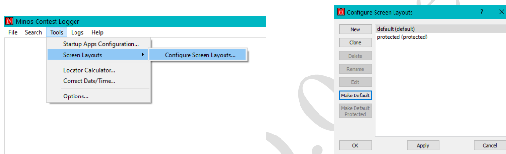
Figure 50 – Invoking the screen layout editor
