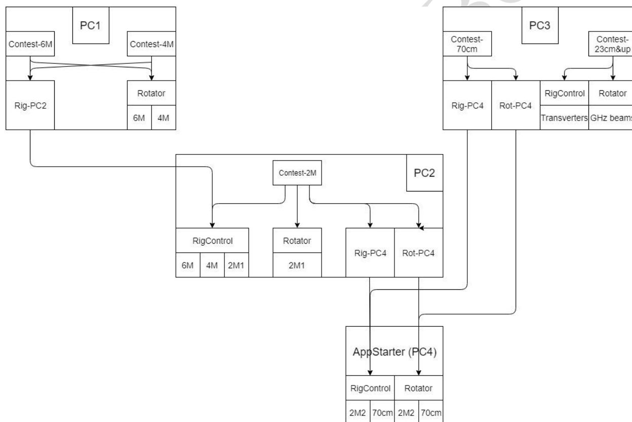
Figure 163 – Example complex configuration.
