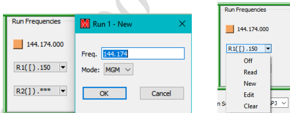
Figure 91 – Storing a run frequency
