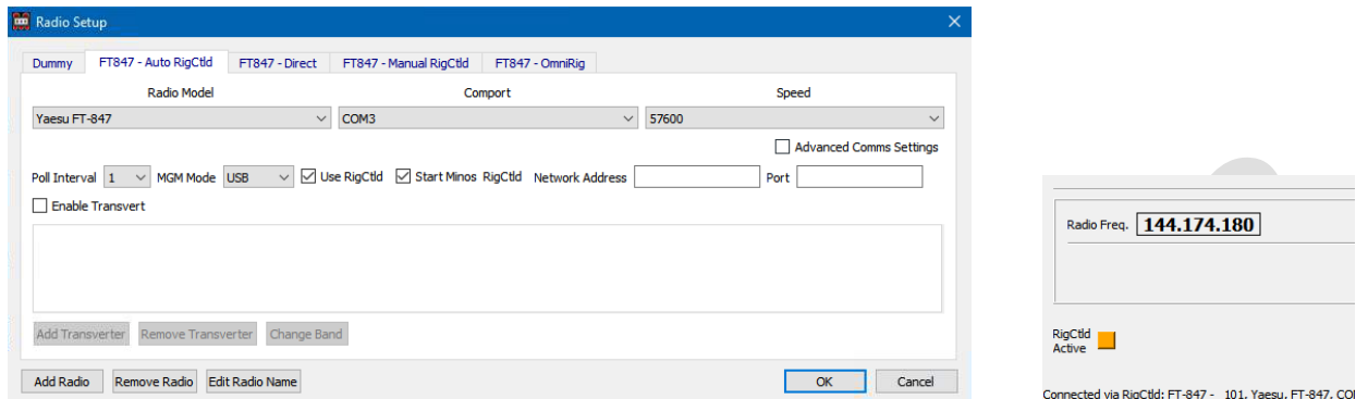
Figure 115 – Defining rigctld connection to Rigcontrol
