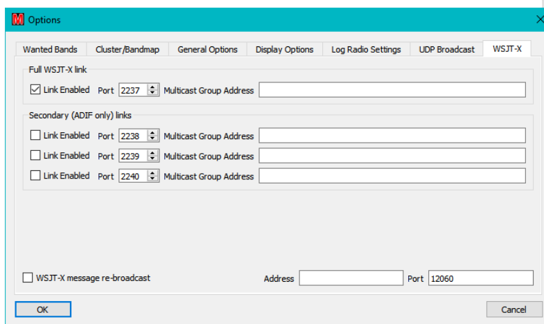
Figure 60 – WSJT-X link configuration
