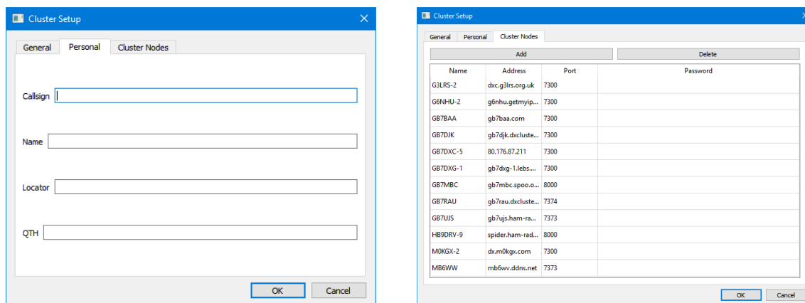
Figure 123 – Cluster Server configuration
