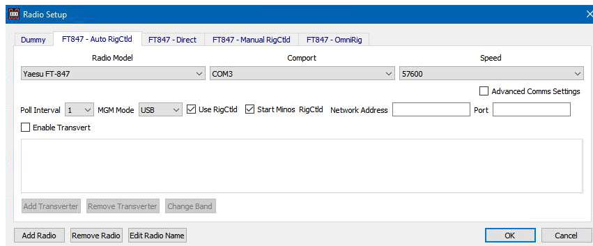
Figure 102 – Defining rigctld connection to Rigcontrol
