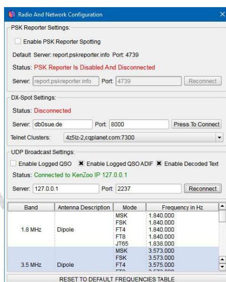
Figure 57 – MSHV configuration
