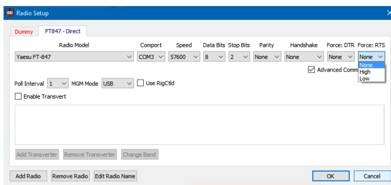
Figure 72 – Advanced comms settings
