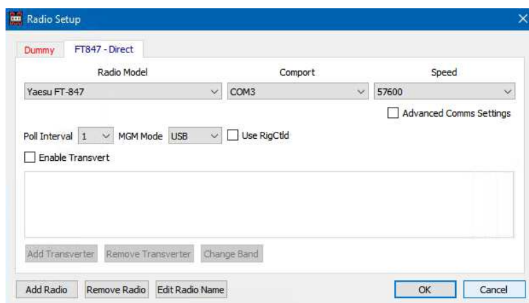
Figure 71 – Simple Configuration of a serial connected rig
