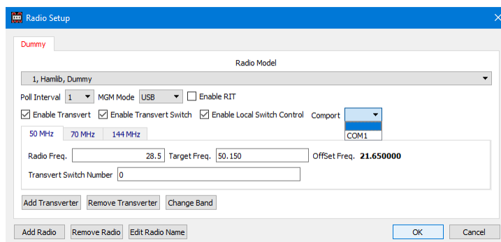
Figure 88 – Defining Local Switch Control port
