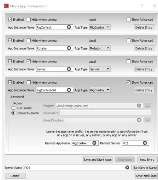
Figure 141 – Configuring two rigs, using remote RigControl
