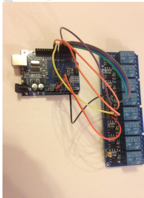
Figure 165 – Arduino and Relay Board
