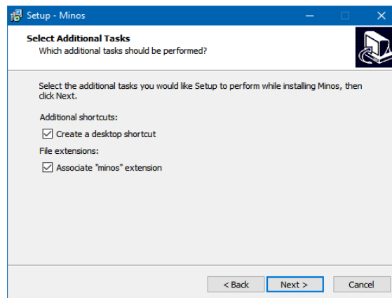
Figure 6 – Additional Tasks
