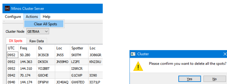
Figure 142 – Clearing spots.
