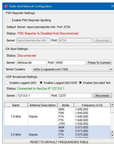
Figure 70 – MSHV configuration
