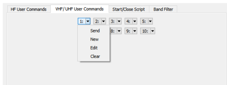
Figure 140 – User Commands
