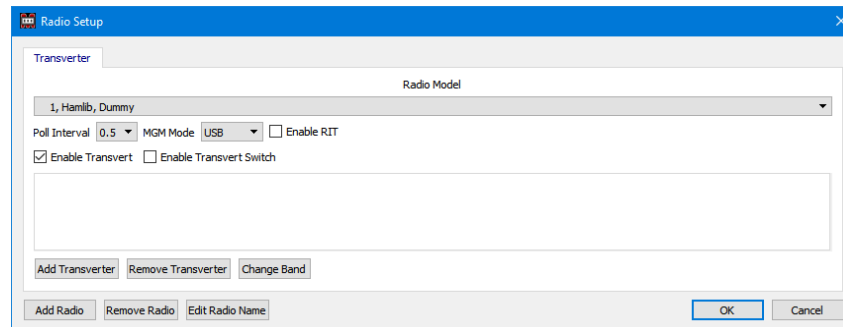
Figure 100 – Transverter configuration
