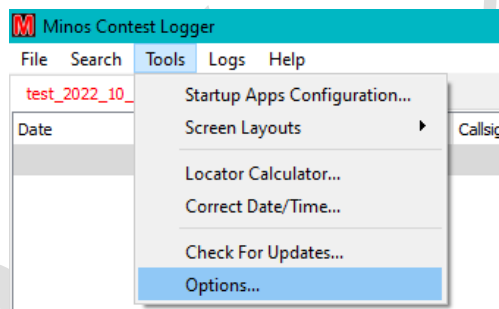
Figure 9 – Tools Menu
