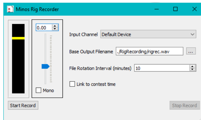
Figure 169 – RigRecorder screen
