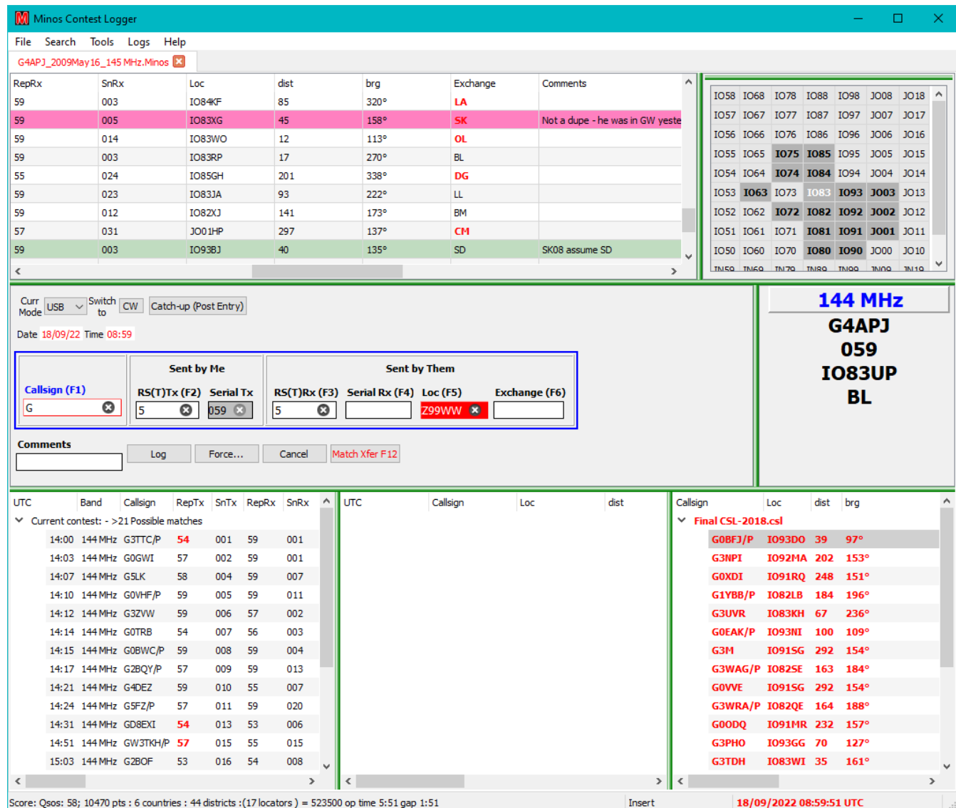
Figure 22 – Colour coding
