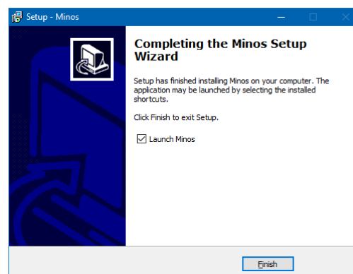
Figure 8 – Installation complete
