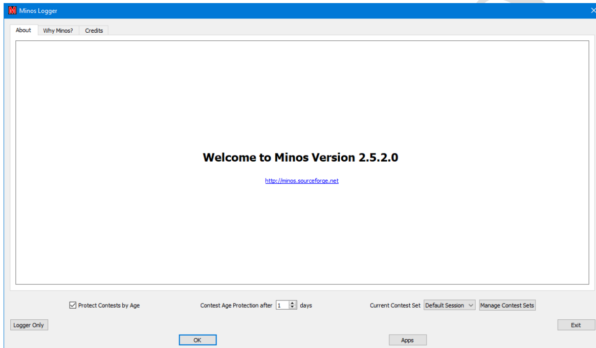
Figure 12 – Welcome screen
