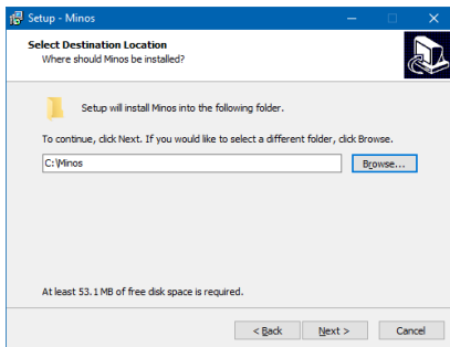
Figure 3 – Target location
