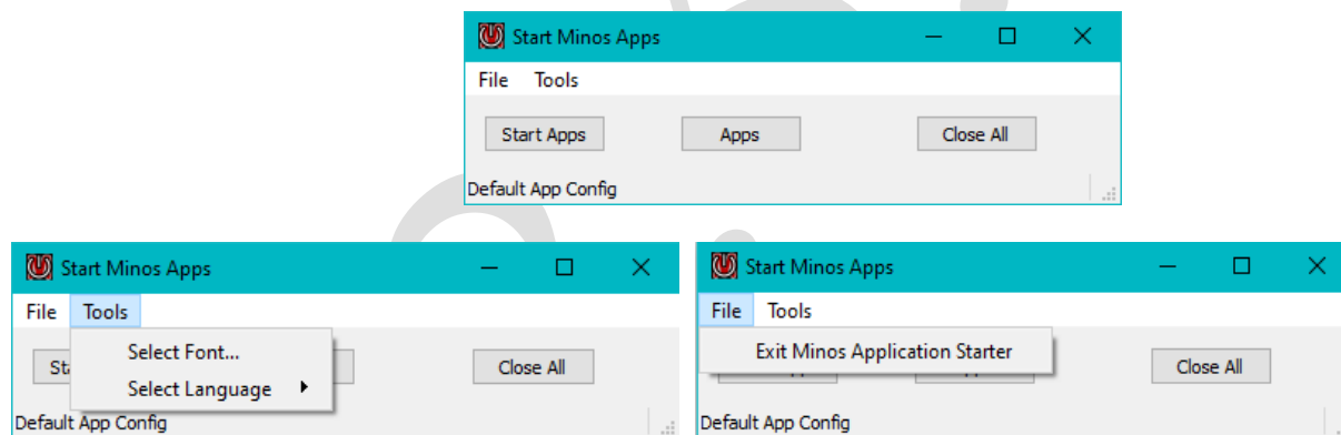
Figure 174 – AppStarter
