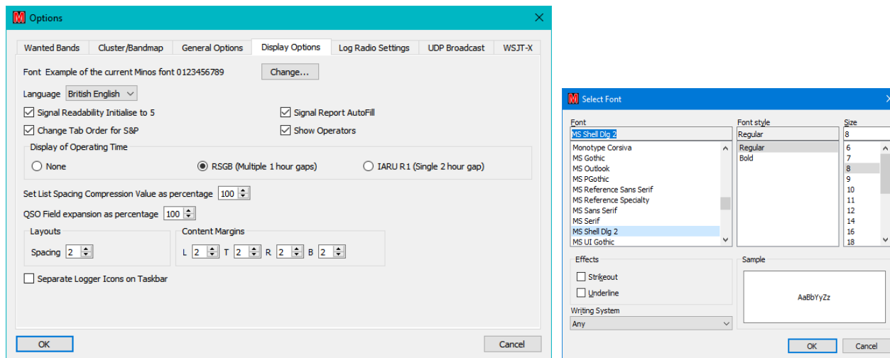
Figure 63 – Font selection
