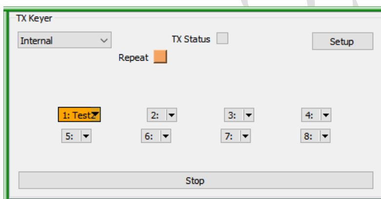
Figure 132 – Keyer activated
