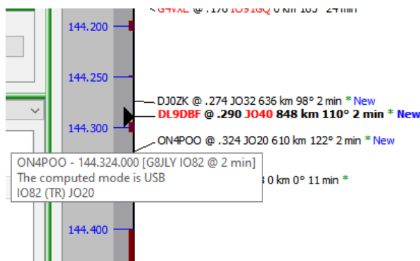
Figure 152 – Marker info
