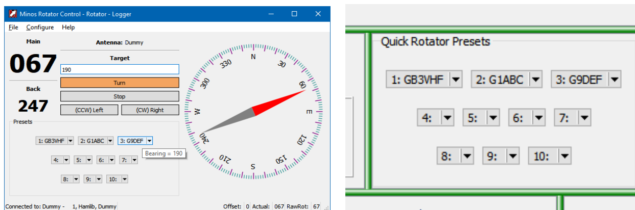
Figure 114 – Configuring pre-sets
