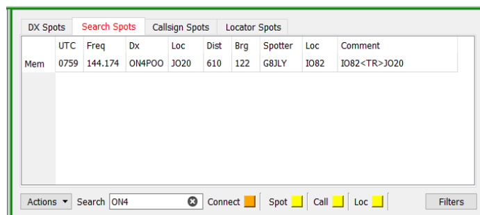
Figure 144 – Search facility
