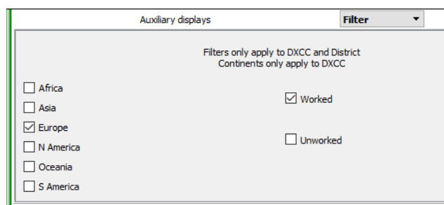
Figure 35 – Statistics Filter
