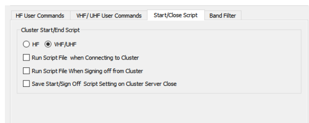
Figure 139 - Start/Close scripts
