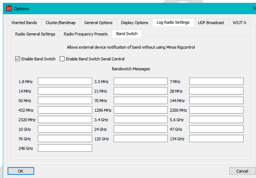
Figure 105 – Bandswitch Messages
