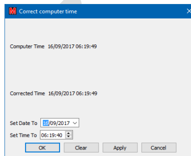
Figure 52 – Clock adjustment
