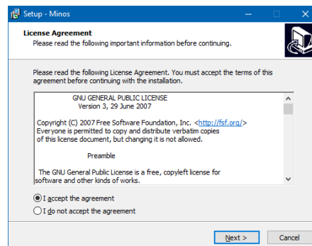
Figure 2 – Licence agreement
