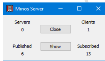
Figure 77 – Server statistics
