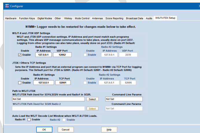
Figure 73 – N1MM+ configuration
