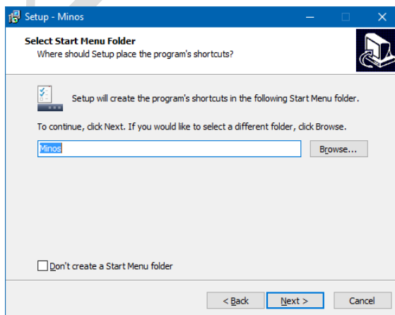
Figure 5 – Start menu
