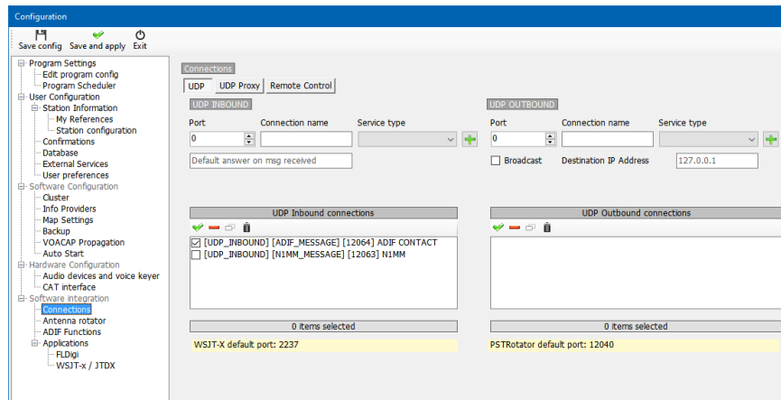
Figure 72 – Log4OM configuration
