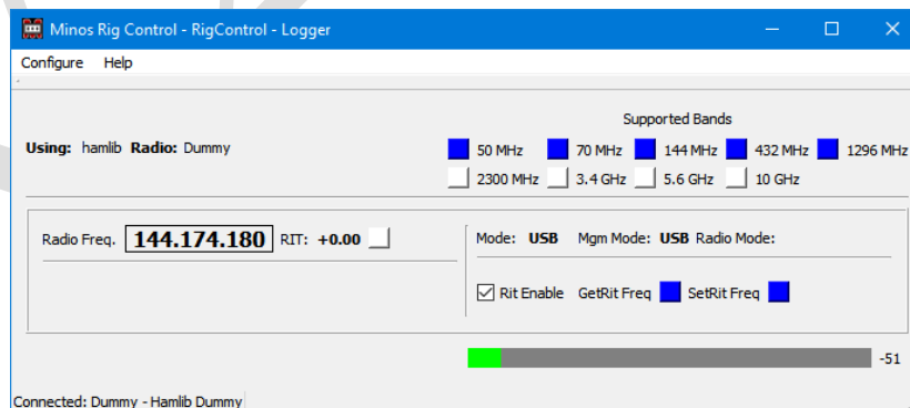
Figure 90 – RigControl operational
