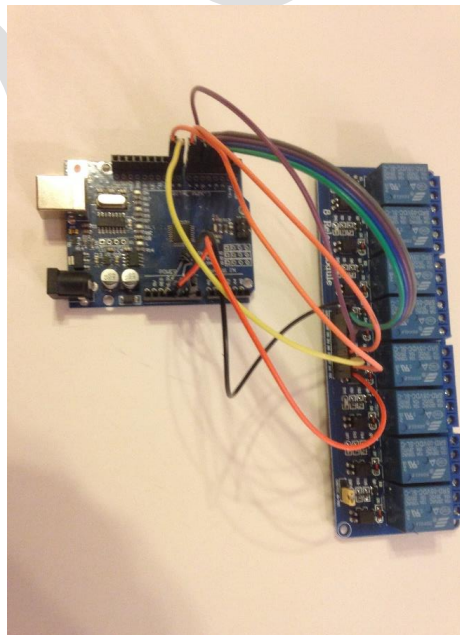
Figure 184 – Arduino and Relay Board
